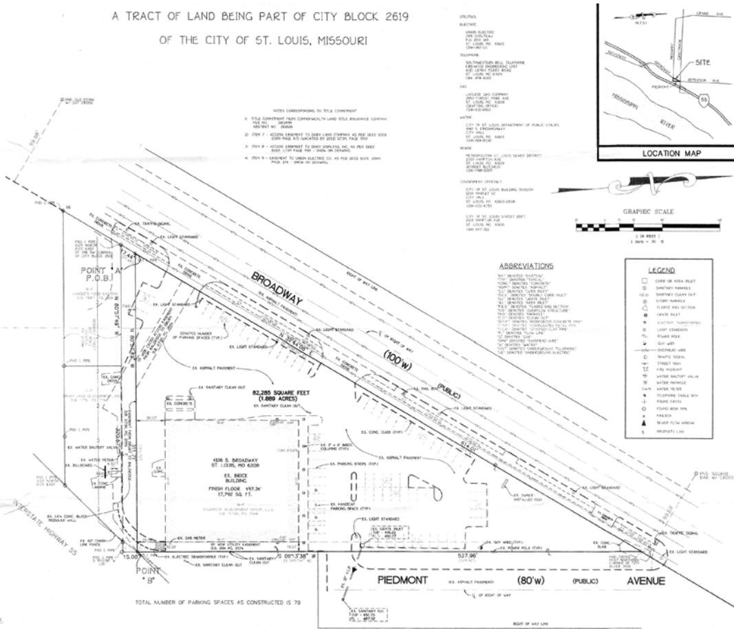
BOUNDARY AND IMPROVEMENT SURVEY
