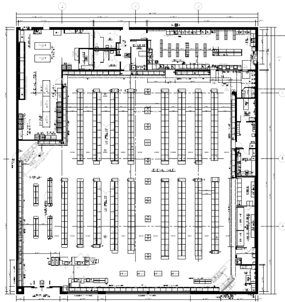
1 FIXTURE FLOOR PLAN 1/8"=1'-0"
